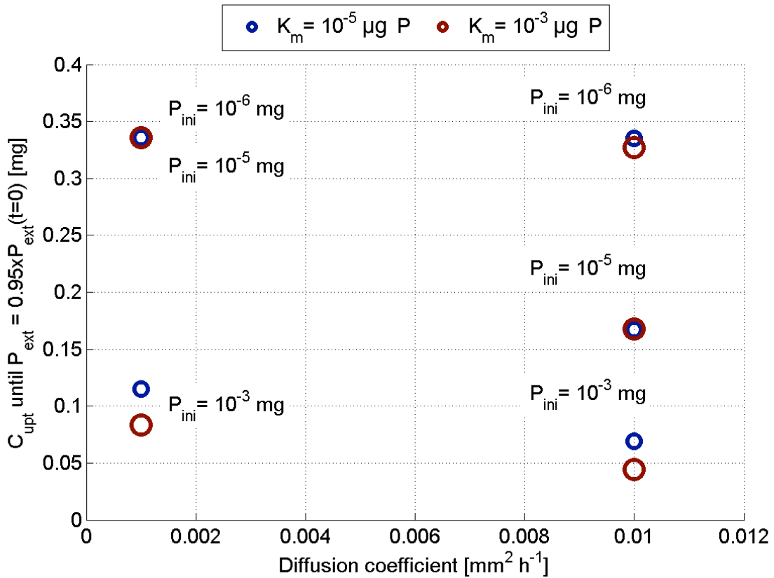
Figure 5-5: C uptake of the fungus until 5% of the initial external P source P_{\text{ext}} is taken up by fungi for all simulated scenarios over the diffusion coefficient D_s . For scenarios in which fungi did not manage to take up 5% of initial P_{\text{ext}} , the fungal C uptake until simulation end was plotted. Since P_{\text{ini}}=10^{-6} and P_{\text{ini}}=10^{-5} did not manage to take up 5% of the initial P_{\text{ext}} for D_s = 0.001 , the values for these scenarios are identical. Different marker sizes represent the two simulated K_m -values.
