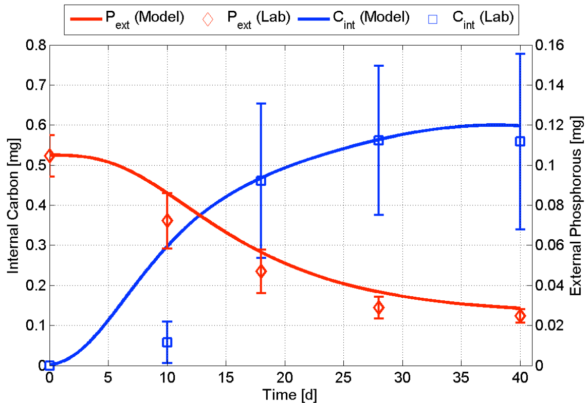
Figure 2-7. Measured and simulated dynamics of carbon and phosphorus.
