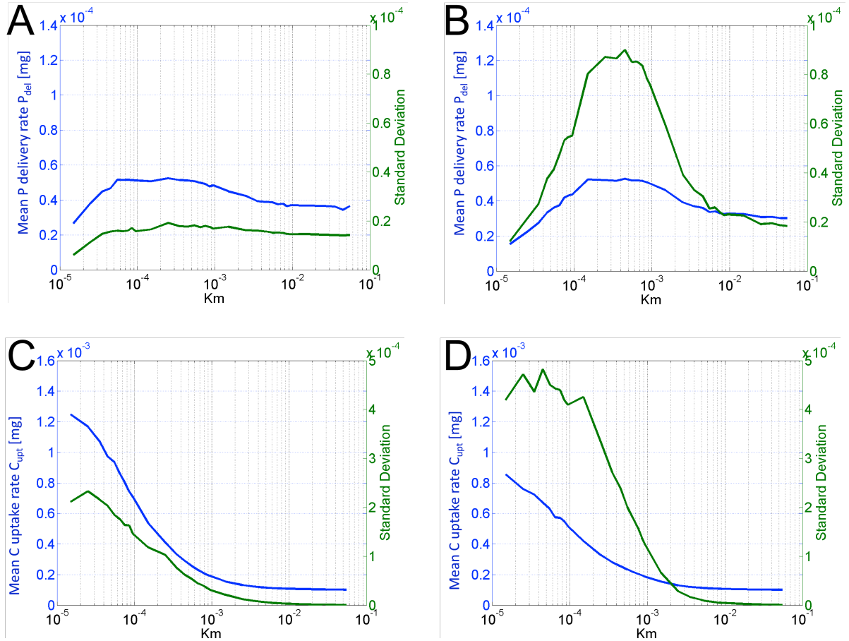
Figure 4-2: Mean (blue curves) and standard deviation (green curves) of the P delivery rate P_{del} (A, B) and fungal C uptake rate C_{upt} (C, D) over K_m . (A,C): Pulse regime 1; (B, D): pulse regime 2.
