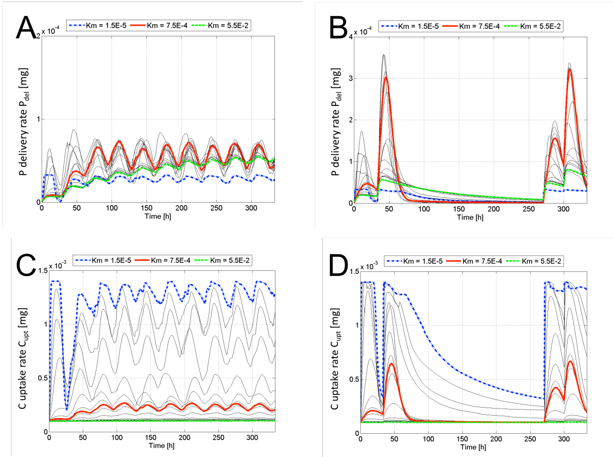
Figure 4-1: Nutrient dynamics for different K_m -values representing three AMF functional types with characteristic nutrient exchange strategies and the two P pulse regimes given in Table 4-1. (A and C): Regular P pulse regime; (B and D): Irregular P pulse regime; (A and B): P delivery to the plant P_{del} ; (C and D) C uptake of the fungus C_{upt} . Colors exemplify K_m values of the parasitic (blue), the intermediate (red) and the mutualistic (green) AMF functional type. Grey lines show K_m values in-between.
