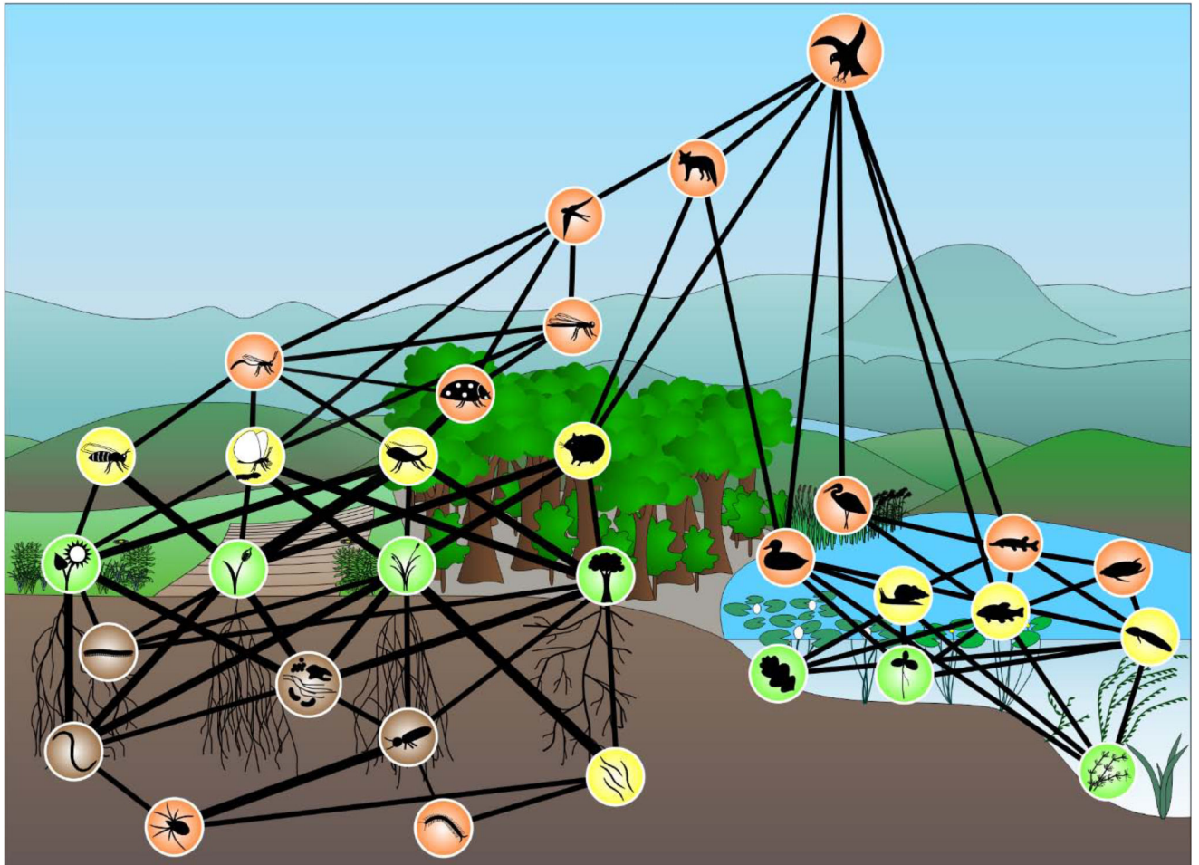
Figure 5. Complex communities link different habitats , a consideration that may facilitate the upscaling of BEF. Conceptual illustration of how multitrophic interactions across ecosystem boundaries can link different ecosystem types and compartments, including above- and belowground compartments, forests and grasslands, as well as terrestrial and aquatic ecosystems. Links between different network modules in these subsystems provide stability of trophic dynamics, matter and energy flow across system boundaries and provide stability of ecosystem function and service delivery (Barnes et al., 2018).
