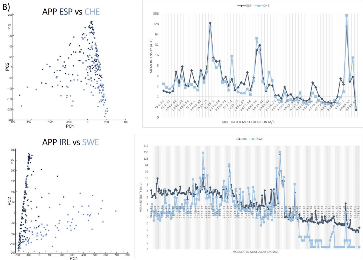
Fig. 2. Principal component analysis of individuals (left graphs) with the lowest and highest modulated molecular ions (MMIs, right graphs) and their corresponding distribution (Log 2 -transformed) in OSR (A) and APP (B). ITA Italy, IRL Ireland, GBR Great Britain, EST Estonia, ESP Spain, CHE Switzerland, and SWE Sweden. Each point represents one haemolymph MFP from an individual bee.
