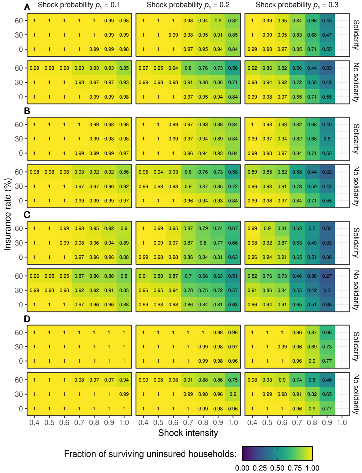
Figure B.7: Fraction of surviving uninsured households among the 20 households that are uninsured in every scenario for idiosyncratic shocks and low level of living costs ( C = 0.7 ) for (A) average degree and rewiring probability as in main text ( N_N = 4 , p_r = 0.2 ), (B) high rewiring probability ( N_N = 4 , p_r = 0.8 ), (C) small average degree ( N_N = 2 , p_r = 0.2 ) and (D) large average degree ( N_N = 8 , p_r = 0.2 ).
