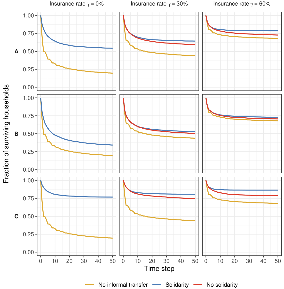
Figure B.3: Fraction of surviving households for different risk-coping instruments and insurance rates ( \gamma = 0\% , \gamma = 30\% , \gamma = 60\% ) with (A) high rewiring probability ( N_N = 4 , p_r = 0.8 ), (B) small average degree ( N_N = 2 , p_r = 0.2 ) and (C) large average degree ( N_N = 8 , p_r = 0.2 ).
