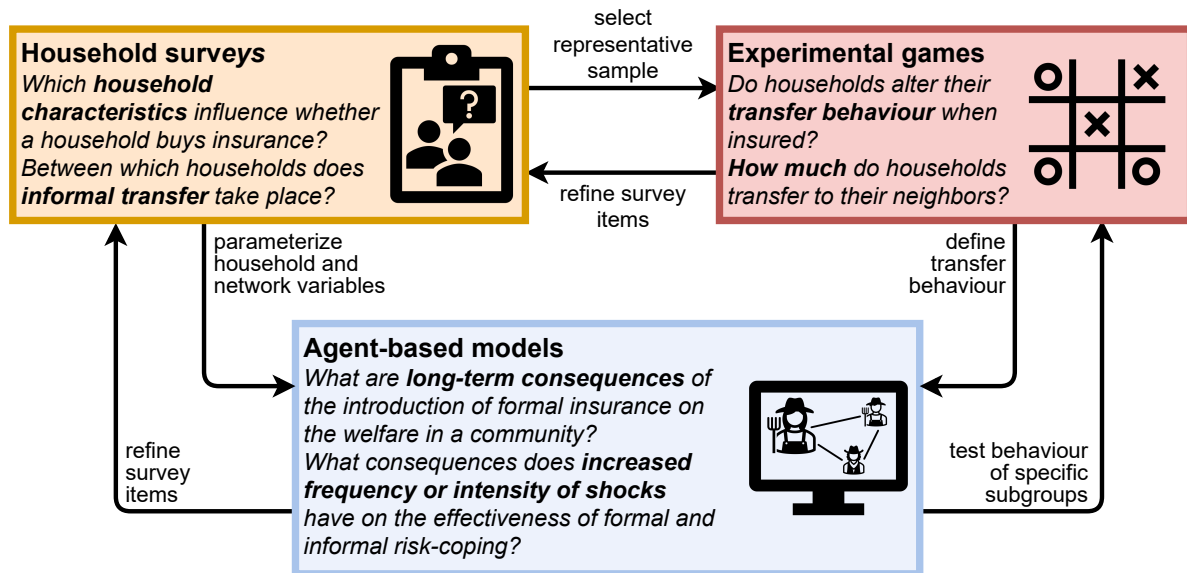
Figure 5.1: Schematic representation of the interplay between empirical data and ABMs to determine the effectiveness of formal and informal risk-coping instruments under climate change
