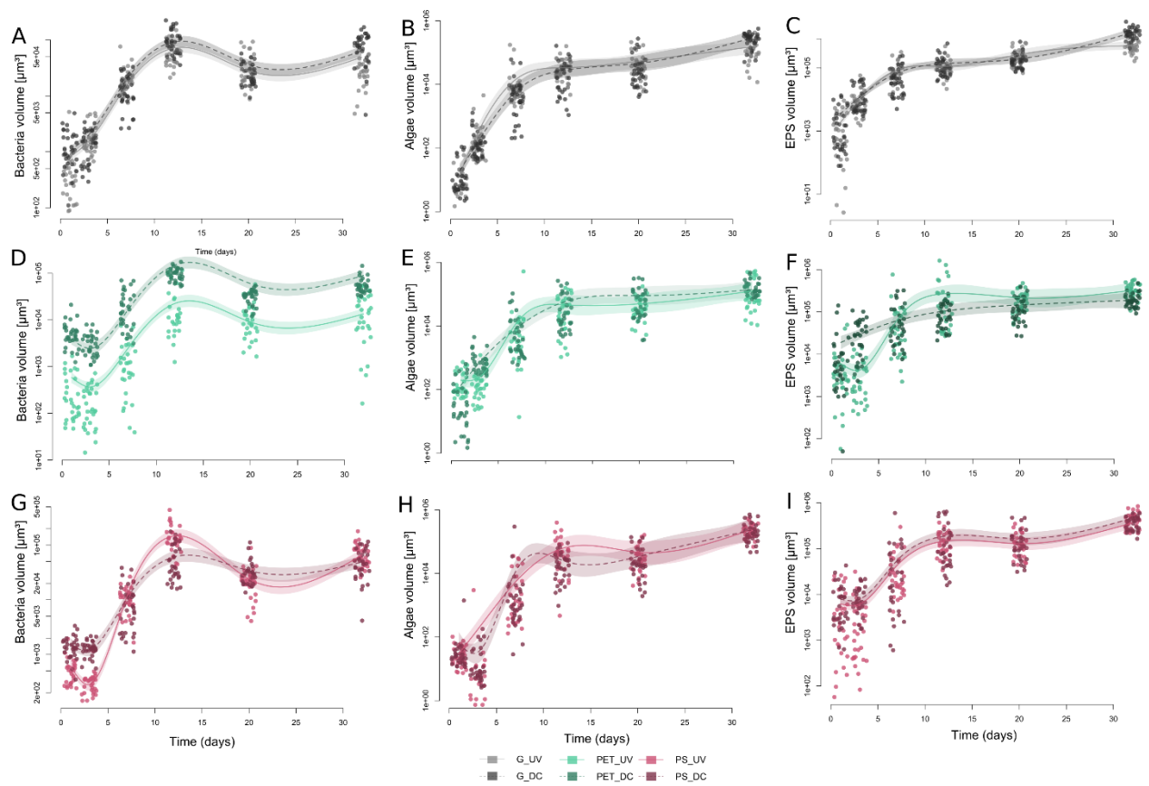
Figure 6 CLSM data fitted with a generalized additive mixed models on the biovolumes [ \mu\text{m}^3 ] of bacteria, algae and EPS matrix comparing weathered (UV) and pristine (DC) substrates over 32 days of incubation. A-C: comparison of glass_DC and UV in the respective biovolumes. D-F: PET_DC shows higher abundance of Prokaryotes than PET_UV, while there is no clear difference in algae biomass. At sampling time 1 and 3 PET_DC showed also higher EPS shares. G-I: Biovolumes of PS_DC and PS_UV. Solid and dashed lines are the predicted means with confidence bands as shaded areas. Y-axis is log-scaled
