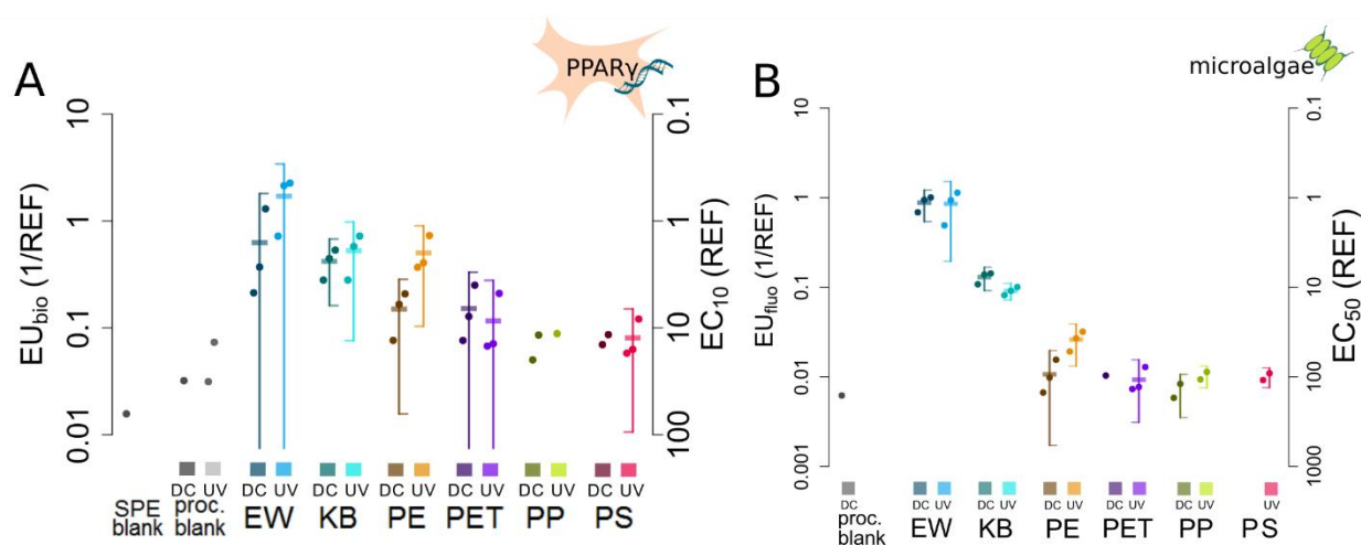
Figure 2.2: Effects of solid phase-enriched microplastic leachates tested in reporter gene and microalgae assays. A: Bioanalytical effect units (EU bio ), defined as the inverse EC 10 (1/REF on left y-axis, REF on right y-axis), measured in the cell-based bioassay PPAR \gamma . B: Effect units for the microalgae endpoint fluorescence (EU fluo ) as the inverse EC 50 (1/REF on left y-axis, REF on right y-axis). Samples are color coded for SPE blanks, procedural blanks, two positive controls (e-waste (EW) and keyboard (KB)) and the four test polymers PE, PET, PP and PS. Dark controls (DC) and UV-treated (UV) samples are presented juxtaposed in darker and lighter shades of the different colors. If all three replicates resulted in measurable effects, the squares represent the mean, whiskers the upper and lower range of the 95 % confidence interval. The absence of symbols implies effect > highest tested concentration (REF 200 and 197 for the cell and microalgae assay, respectively)
