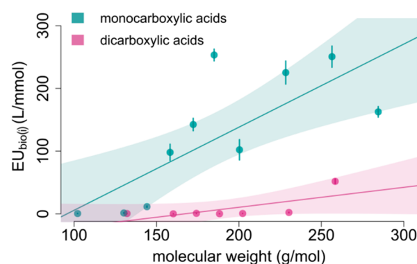
Figure 2. Effect units ( EC_{bio(i)} = 1/EC_{10(i)} ) elicited in the PPAR \gamma assay by mono- and dicarboxylic acids of increasing chain length (CS, C7–C12, C14, C16, C18). Monocarboxylic acids showed a significant correlation between molecular weight and target activation ( R^2 = 0.66 , p < 0.01 ), which was nonsignificant for the dicarboxylic acids (solid line represents the respective regression line with the shaded area as the 95% confidence band).
