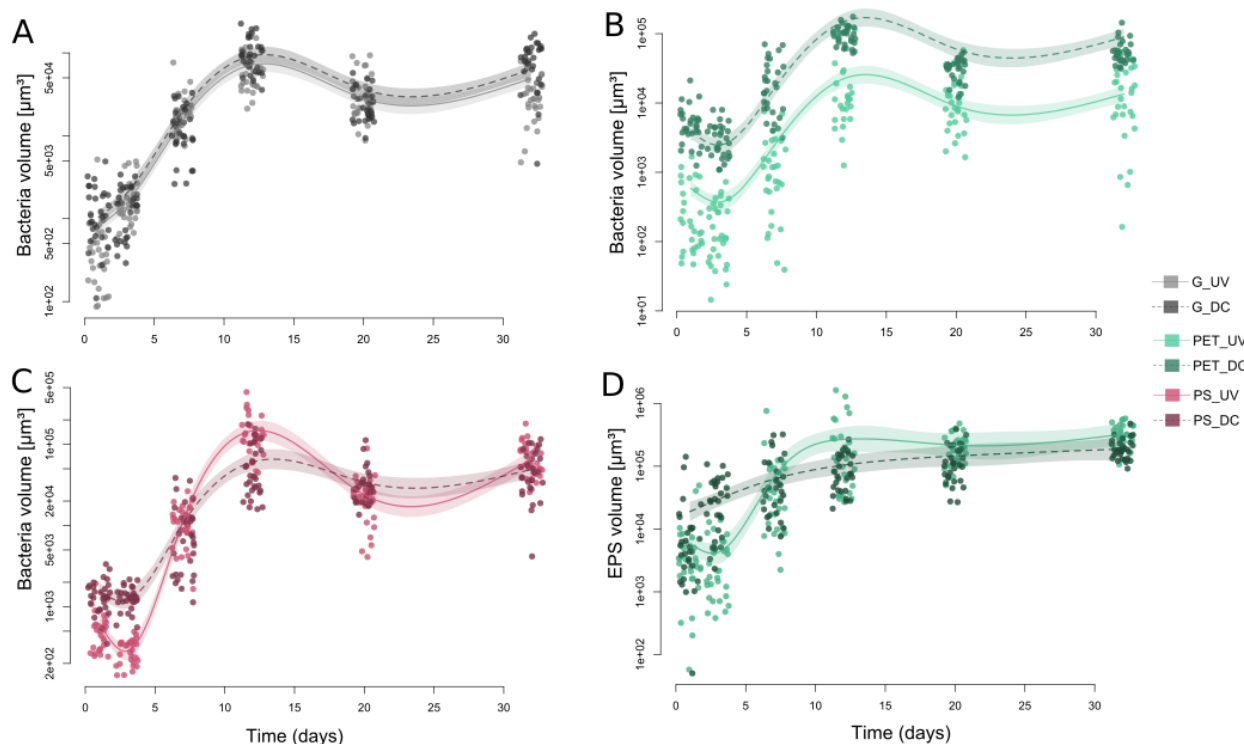
Figure 3.8: Generalized additive mixed models (GAMMs) on the biovolumes [ \mu\text{m}^3 ] of bacteria ( A-C ) and extracellular polymeric substances (EPS) ( D ) over 32 days of incubation time including weathering (DC and UV treatment) as a factor. A: comparison between bacteria biovolumes on glass_DC and glass_UV with no differences in growth. B: PET_DC showed higher abundance of prokaryotes than PET_UV. C: bacteria biovolumes of PS_DC and PS_UV with differences at early time points. D: EPS volumes measured for the substrates PET_DC and PET_UV. Solid and dashed lines are the predicted means with 95 % confidence bands of the mean as shaded areas and y-axis is log-scaled.
