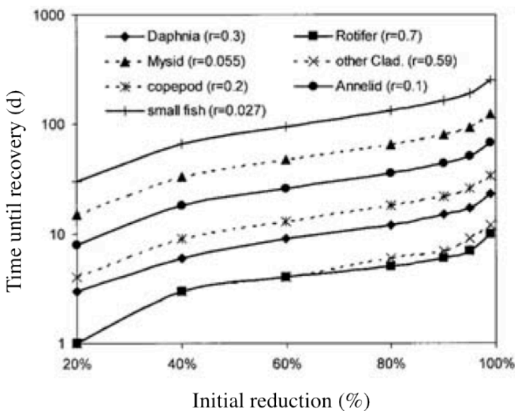
Fig. 1.2: Time until population recovery depending on the initial reduction, modified after Barnthouse (2004).
