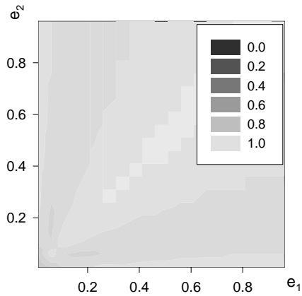
Figure 7: Same as Fig. 3, but with z_1 = z_2 = 1.5 .
